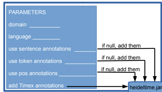
Figure 1: Architecture of the HeidelTime GATE wrapper
