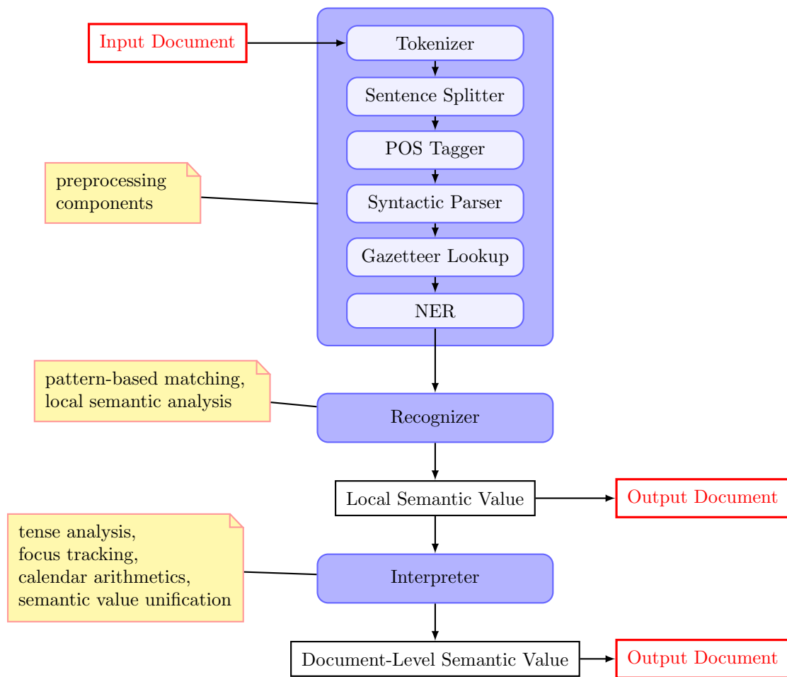
Figure 7.1: Pipeline-based processing in the DANTE system.
