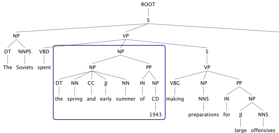
Figure 5.9: A constituency tree for a sentence containing two temporal expressions in a conjunction structure with an ellipsis.
