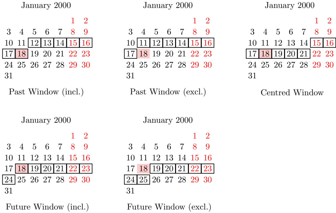
Figure 6.5: Window-based heuristics for the interpretation of weekday names.
