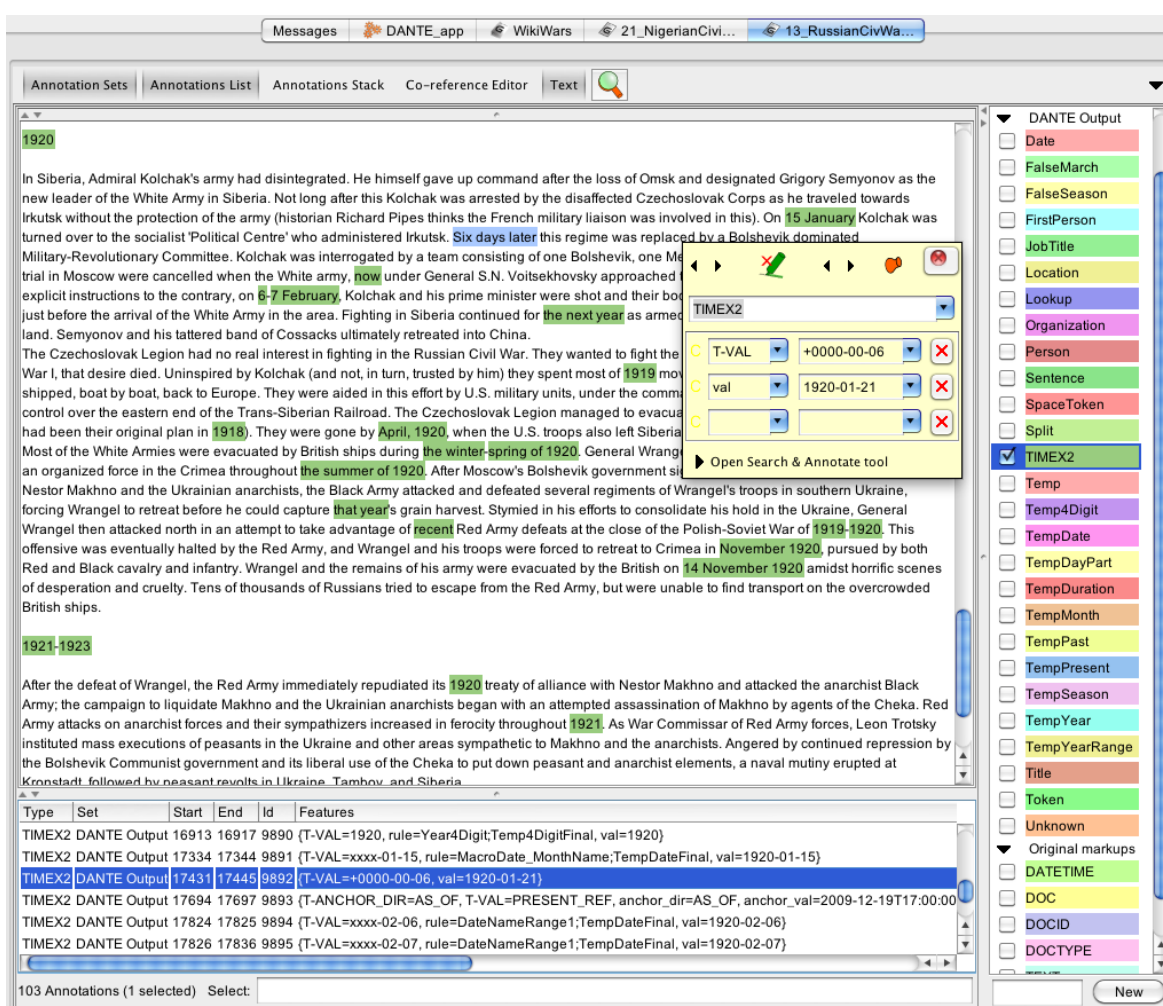
Figure 7.4: A view of GATE Developer with a document processed using DANTE.
