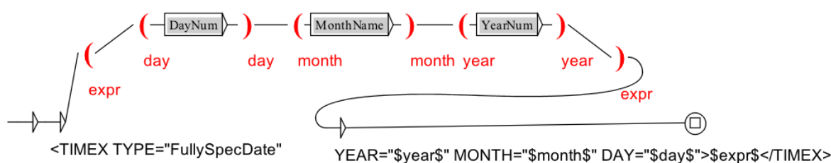
Figure 2.10: A finite-state transducer (FST) recognizing a fully-specified date in DayNum MonthName YearNum format and generating a TIMEX tag around the matched expression with attributes expressing the local semantics of the expression.
