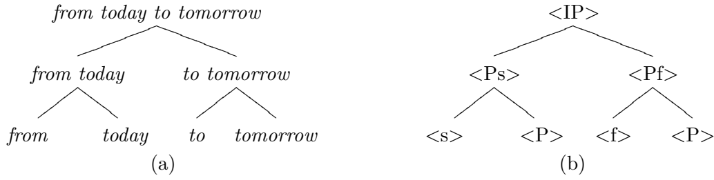
Figure 2.6: An example of expression constituents (a) and their concepts (b) in the formalism of Mizobuchi et al. (1998).
