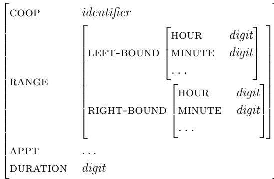
Figure 2.4: The AVM used by Busemann et al (1997) to represent temporal information about a meeting.
