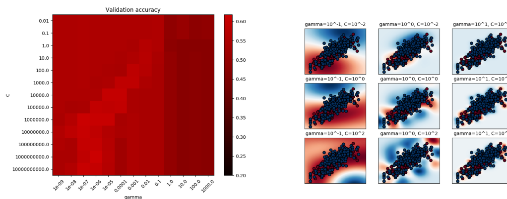
Figure 4. Tuning parameters for the RBF SVM
